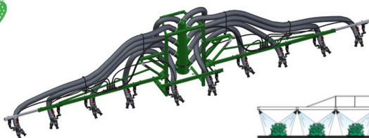
Manual Folding Pneumatic Air Boom
